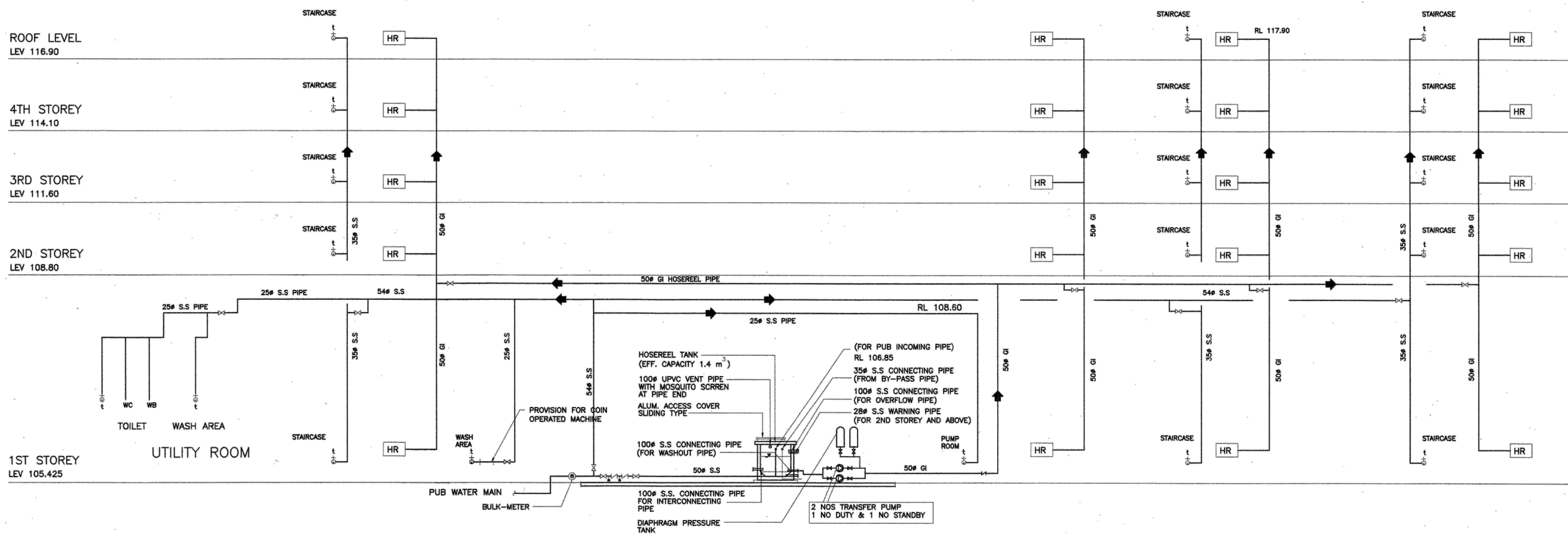
TYPICAL MULTISTOREY CARPARK (MSCP 769A)
